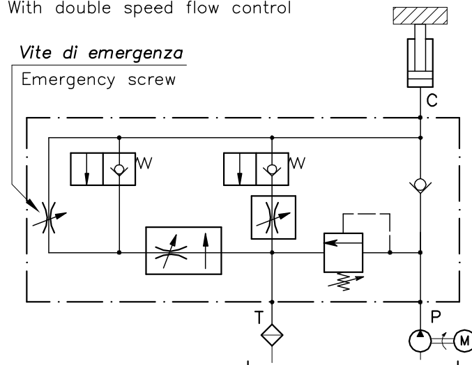
VC-DC-12R-LVE-SM-14
